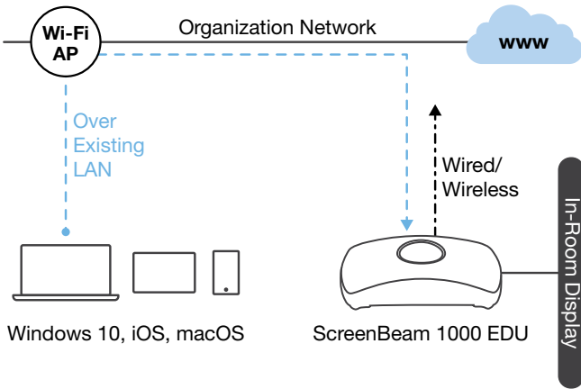
Figure 3 Clients devices use wireless display over the infrastructure network
